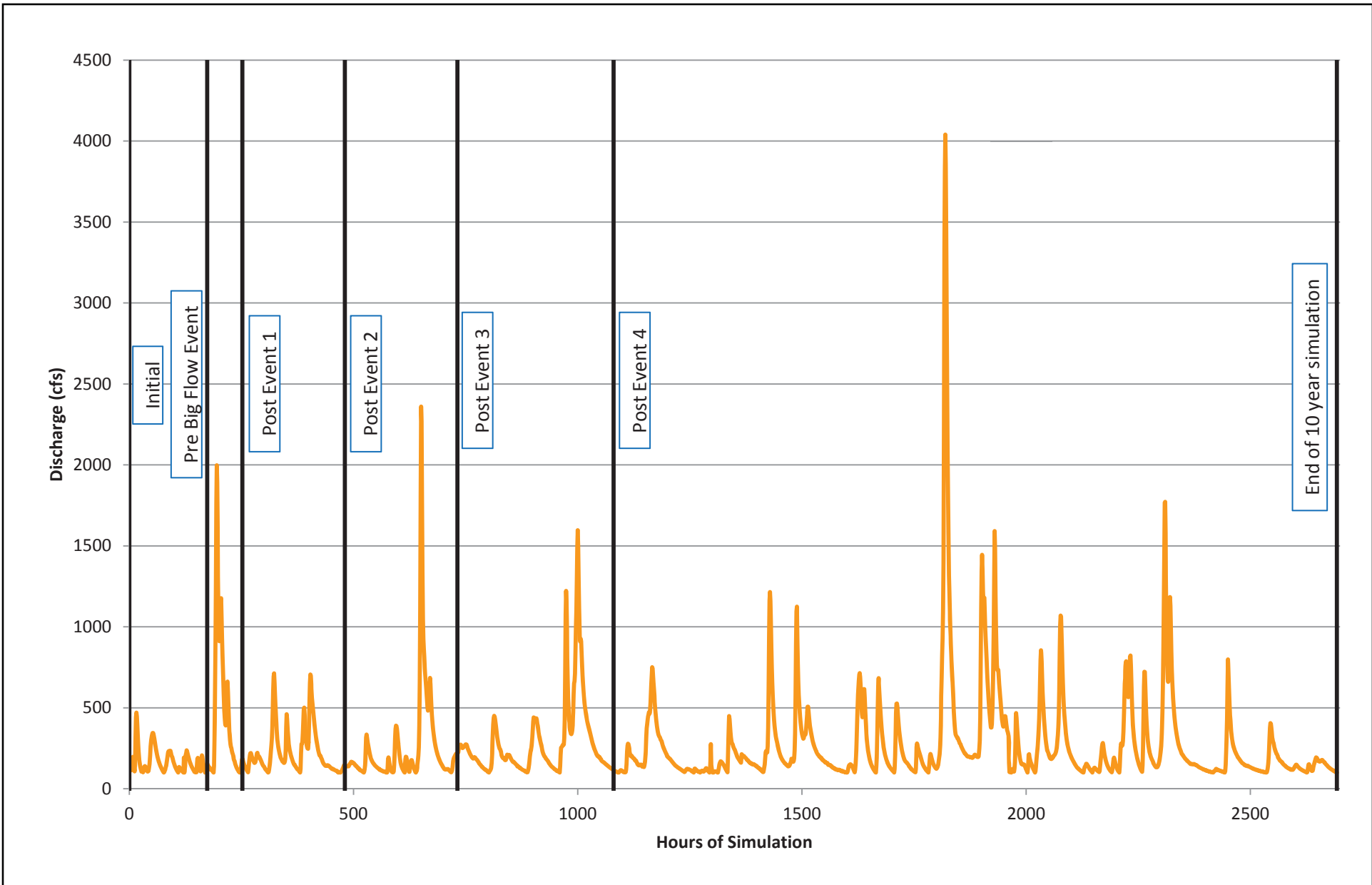
Figure A. Sediment Transport Simulation Hydrograph
