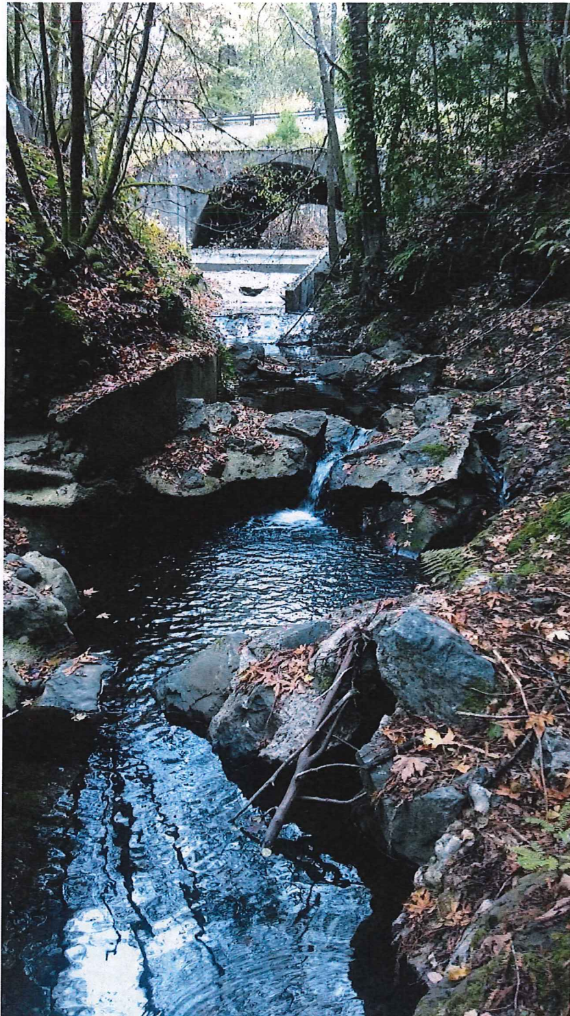
Photo 5) ) November, 18 th 2014 (During extremely low flow drought conditions). Looking Upstream at the three failing boulder weirs and the road crossing, culvert and apron, and fish ladder in the background. Photo provided by RCD.
